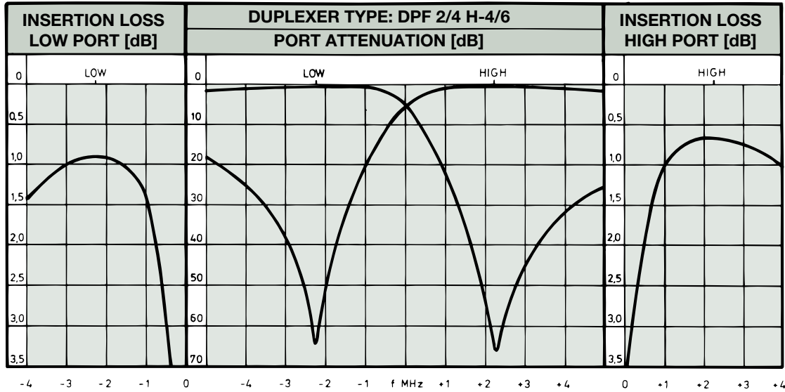
TYPICAL RESPONSE CURVES @ 4.5 MHz DUPLEX SPACING:
