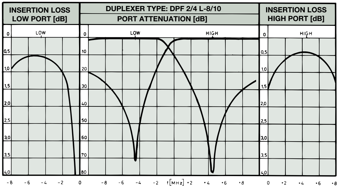
TYPICAL RESPONSE CURVES @ 9 MHz DUPLEX SPACING:
